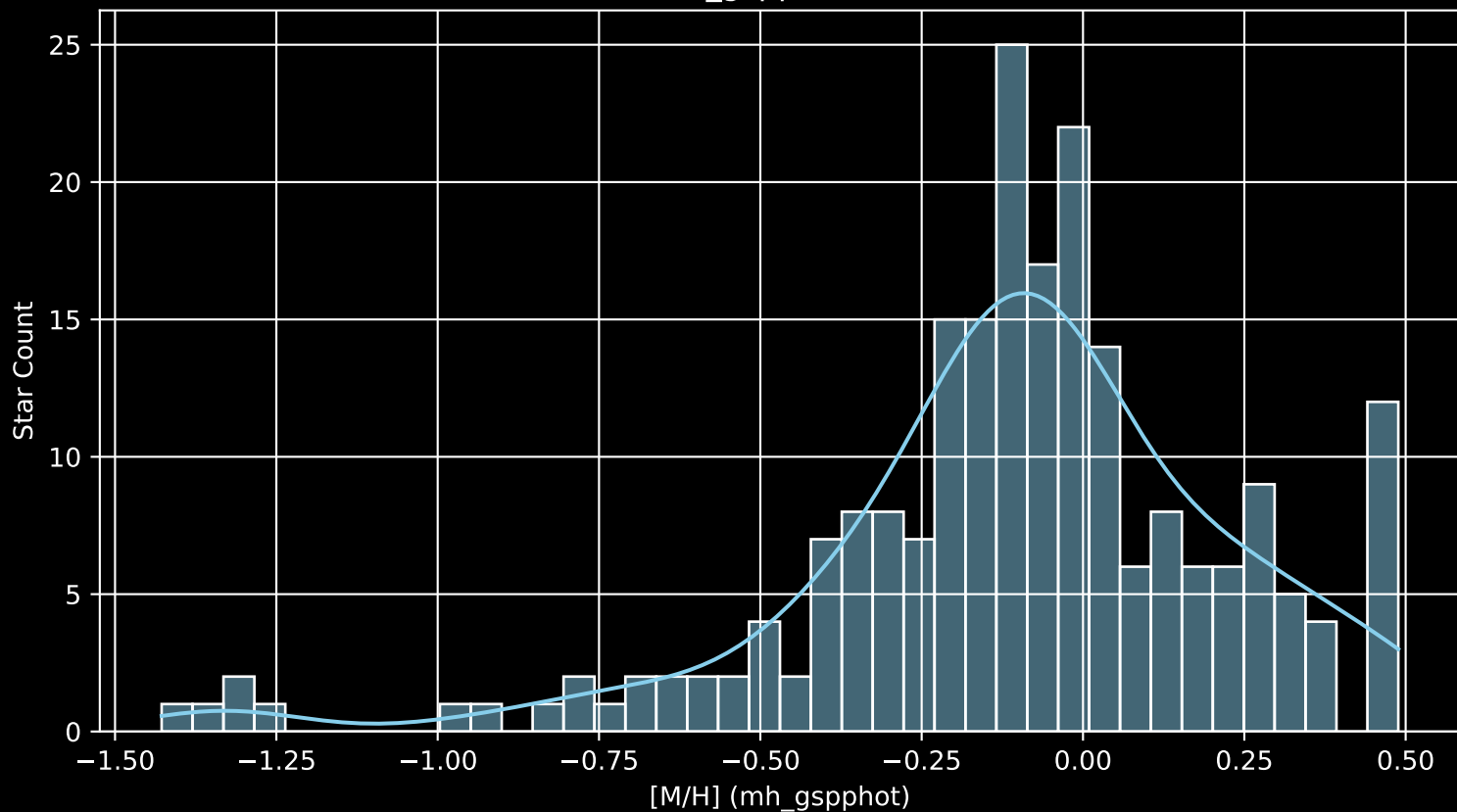
APOGEE DR17 Field: [261-27-C [M/H] (mh_gspphot) (n= 219)
