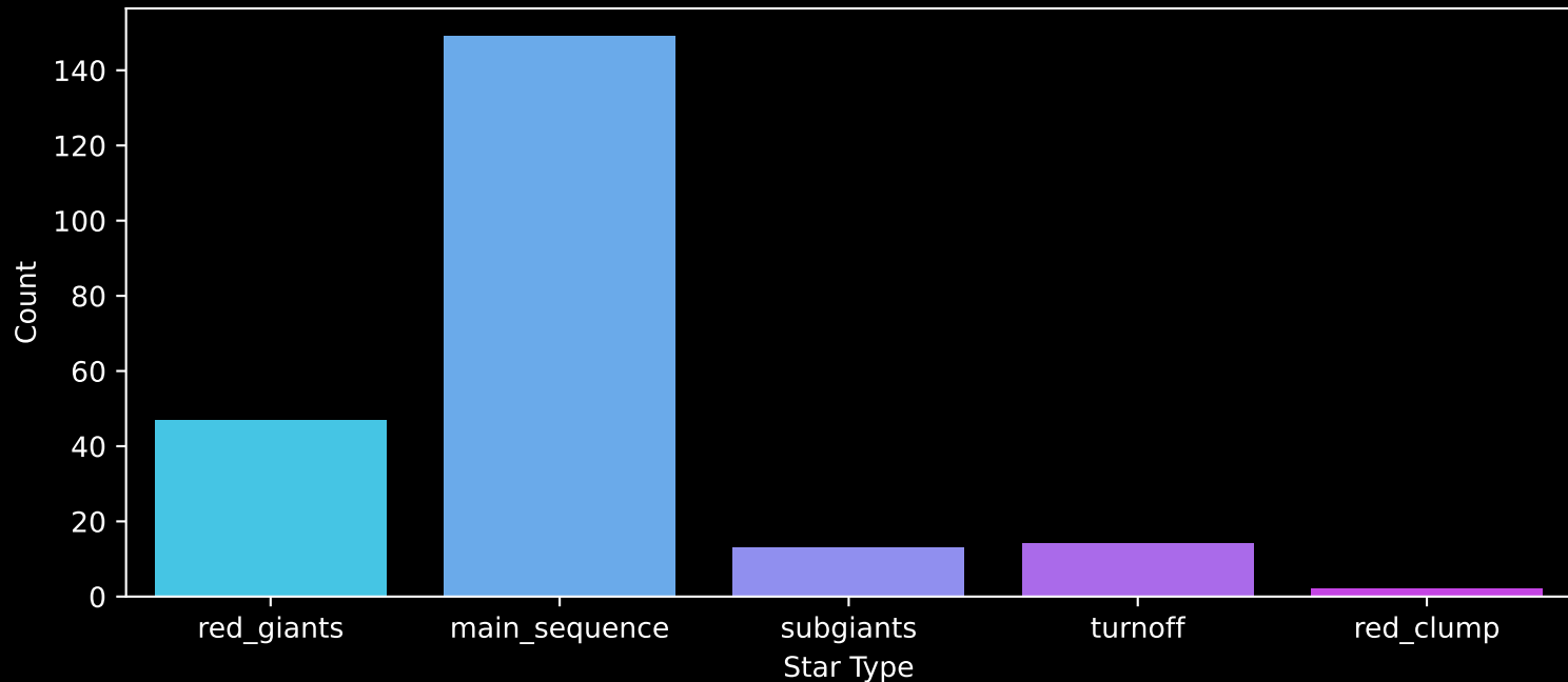
APOGEE DR17 Field: [261-27-C] Count plot of Star Type
