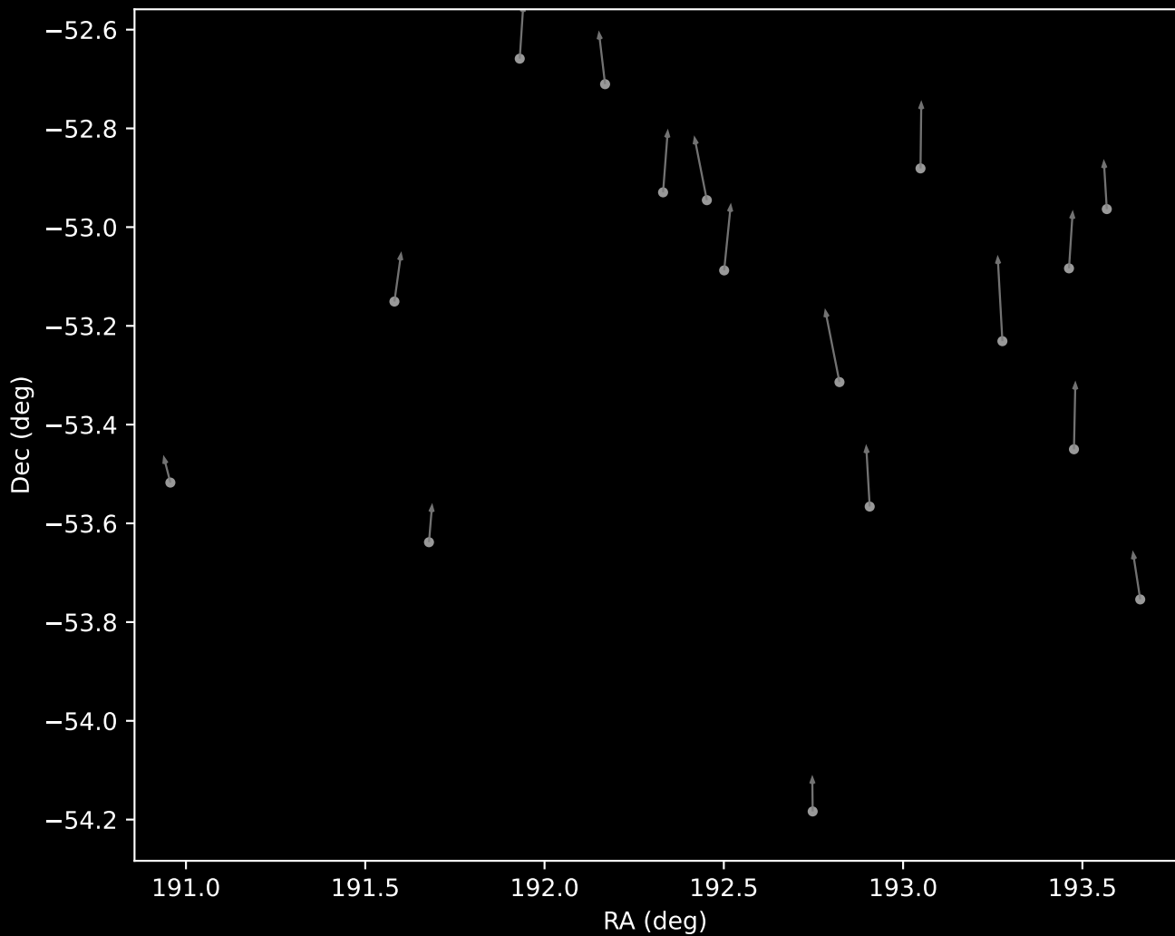
APOGEE DR17 Cluster 14 Proper Motion Vectors (n=17)
