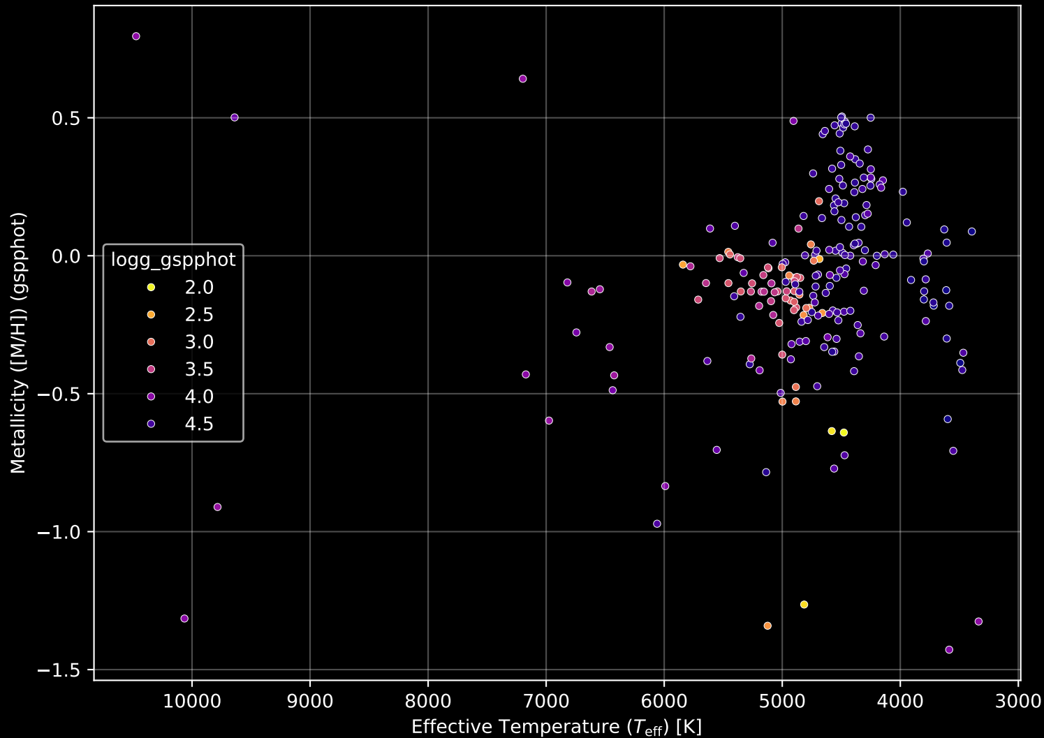
APOGEE DR17 Field: [261-27-C] Stellar Population Parameters (n= 225)
