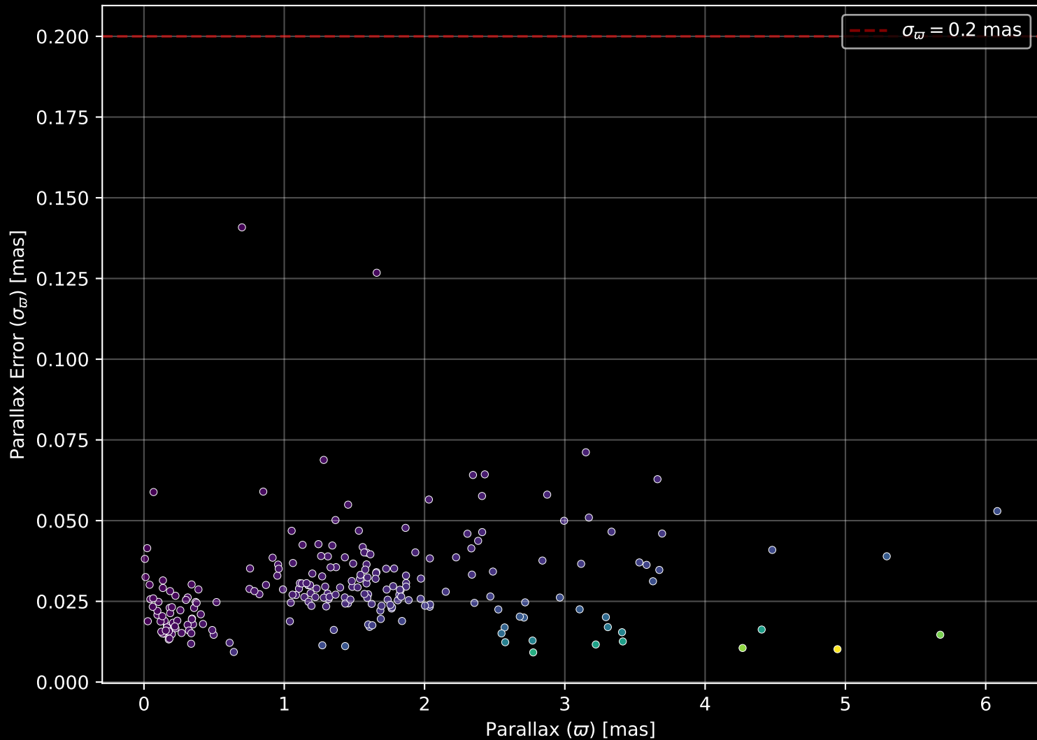
APOGEE DR17 Field: [261-27-C] Parallax Quality (n= 225)
