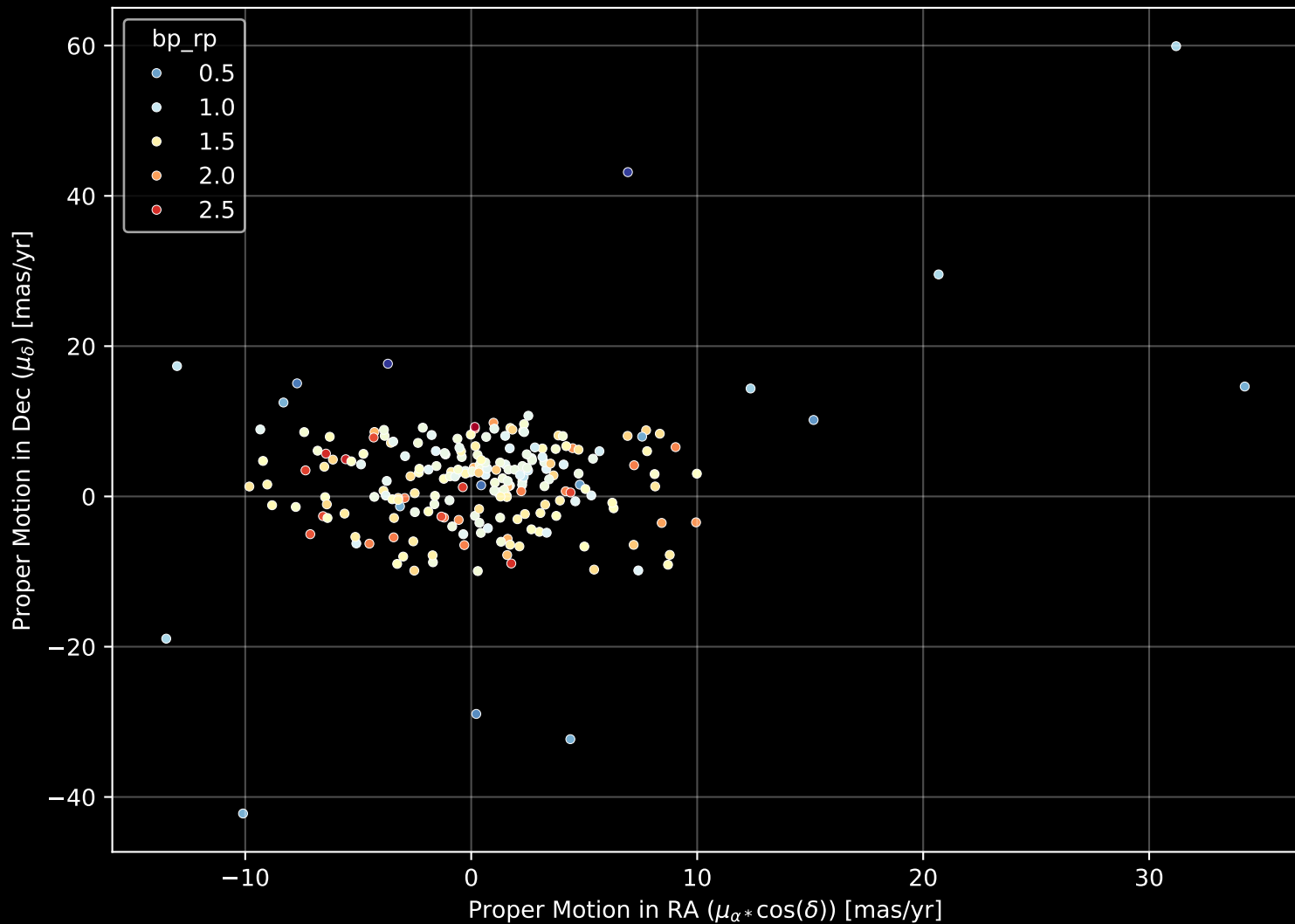
APOGEE DR17 Field: [261-27-C] Proper Motion Diagram (n= 225)
