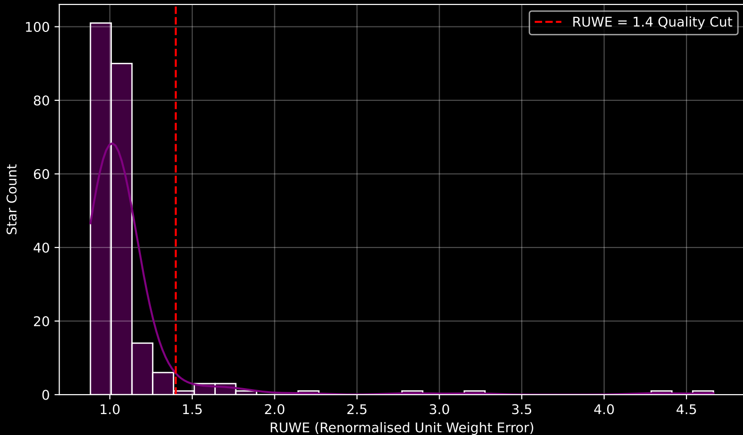
GAPOGEE DR17 Field [261-27-C] RUWE Distribution (n= 224)
